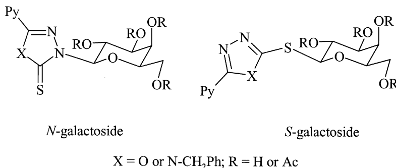
Scheme 3. Conceivable isomeric galactosides.
