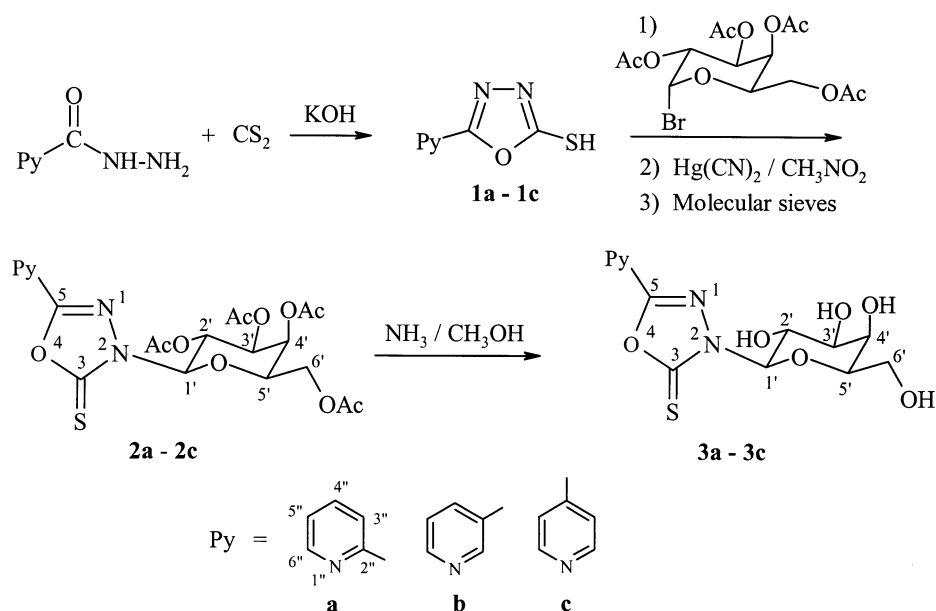
Scheme 1. Synthesis of oxadiazole-2-thione galactosides.
