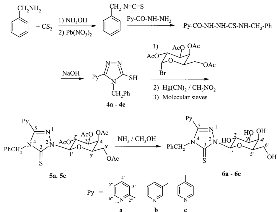
Scheme 2. Synthesis of triazole-3-thione galactosides.
